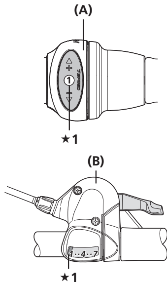
★1 Set to 1 (A) REVOSHIFT lever (B) RAPIDFIRE Plus shifting lever
